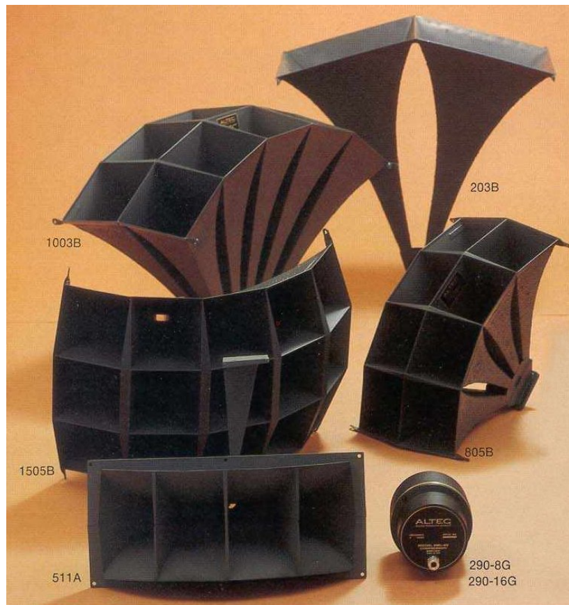
Various Altec-Lansing Multi-Cellular Horns & Horn Driver
