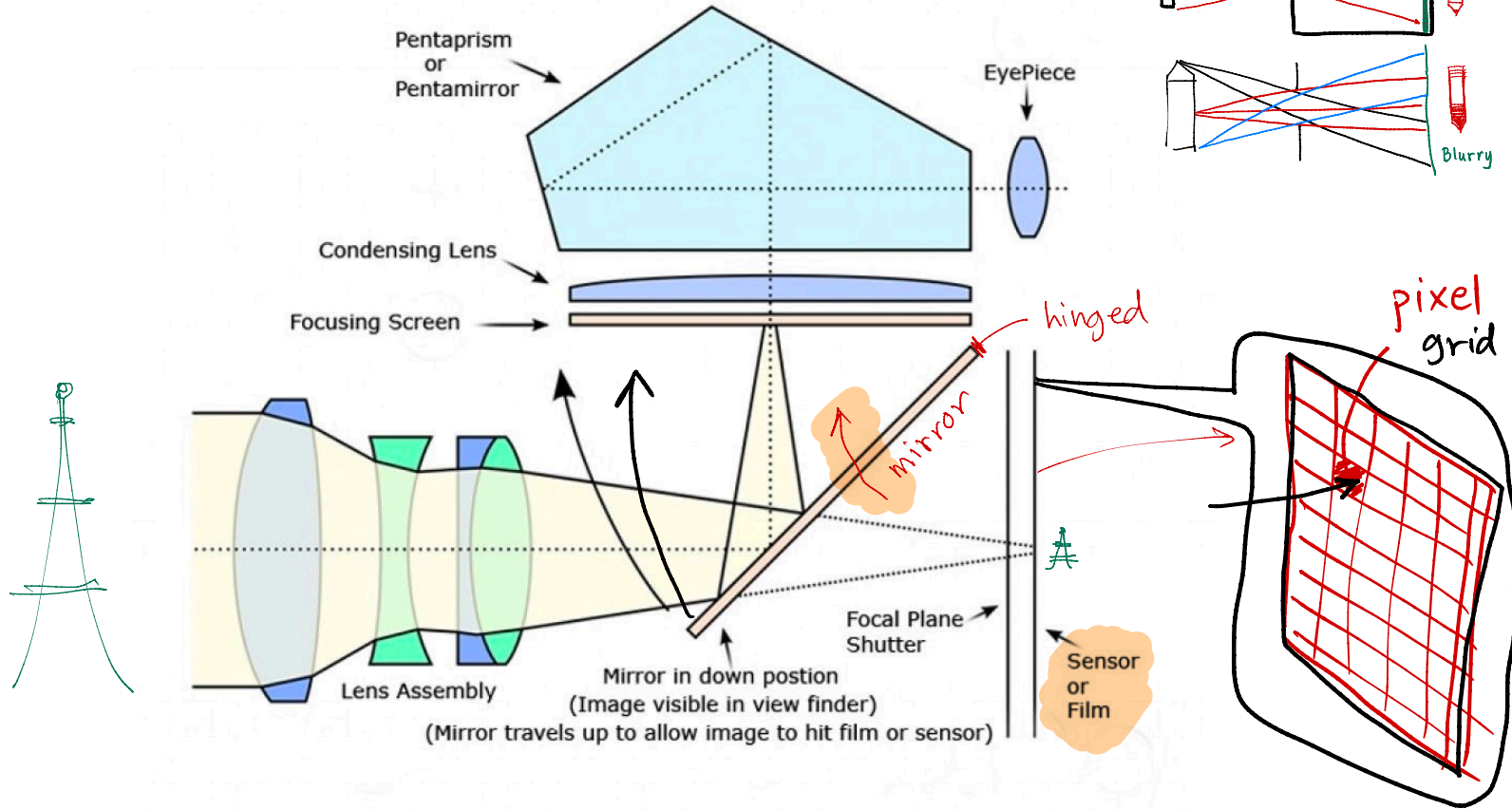
Diagram of most SLR cameras
