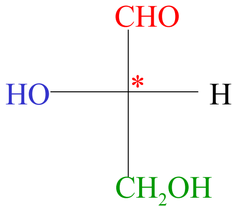
(-)-glyceraldehyde
