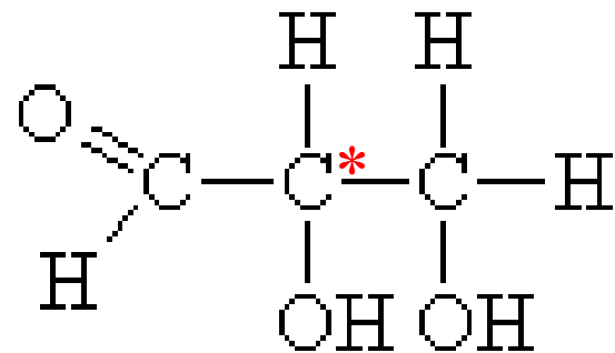
(-)-glyceraldehyde
