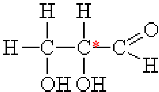
(+)-glyceraldehyde
