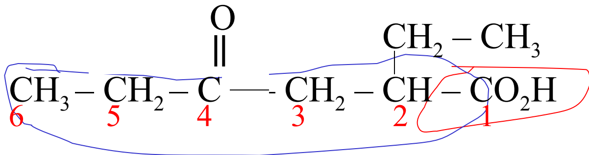
2-ethyl-4-hydroxyhexanoic acid
