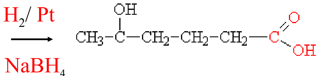
5-hydroxyhexanoic acid
