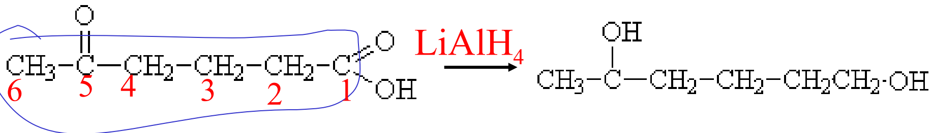
5-oxohexanoic acid
