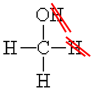
methanol
