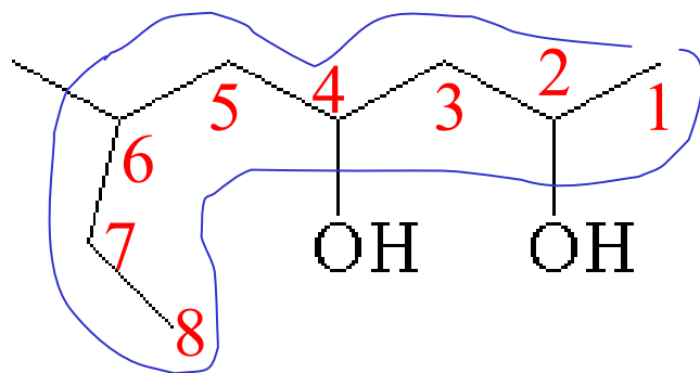
6-methyl-2,4-octanediol
