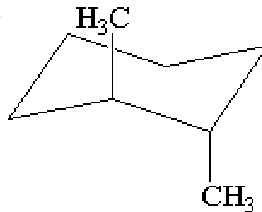
trans -1,2-dimethylcyclohexane
