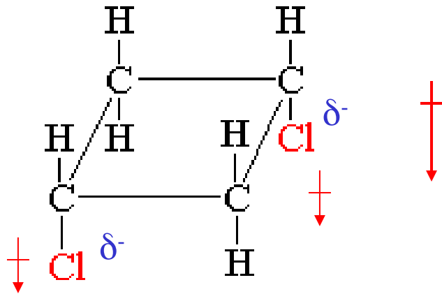
cis -1,3-dichlorocyclobutane
