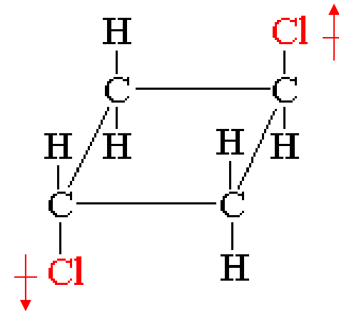
trans -1,3-dichlorocyclobutane
