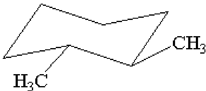
trans -1,2-dimethylcyclohexane
