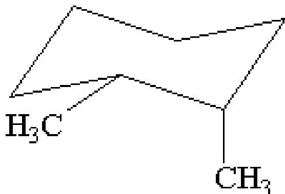
cis -1,2-dimethylcyclohexane
