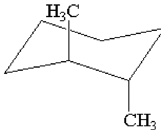
trans -1,2-dimethylcyclohexane
